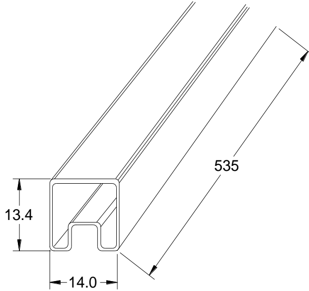
Tube: 535*13.4*14.0mm
